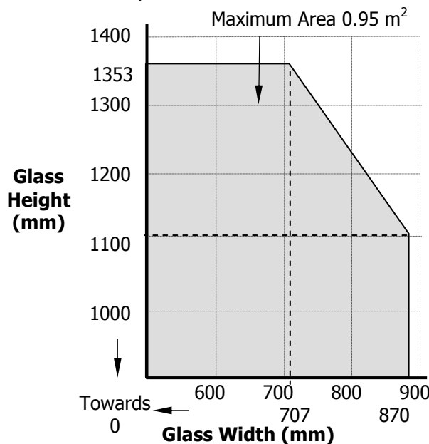
Figure 14. Maximum Permitted Glass Dimensions
