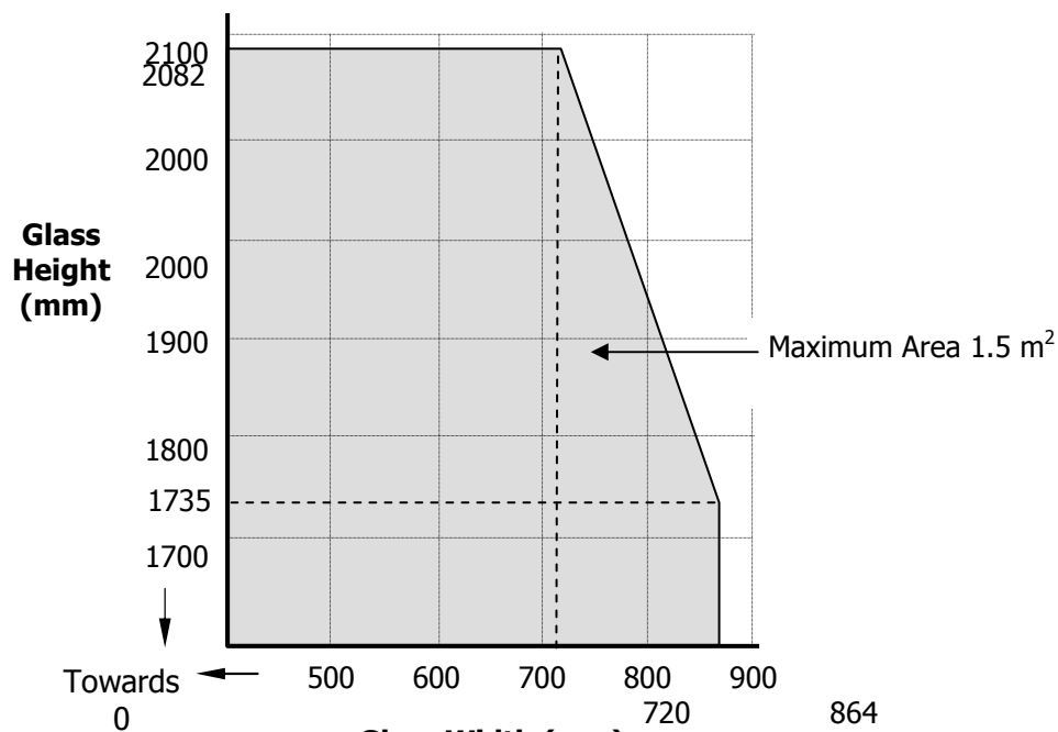
Figure 16. Maximum Permitted Glass Dimensions
