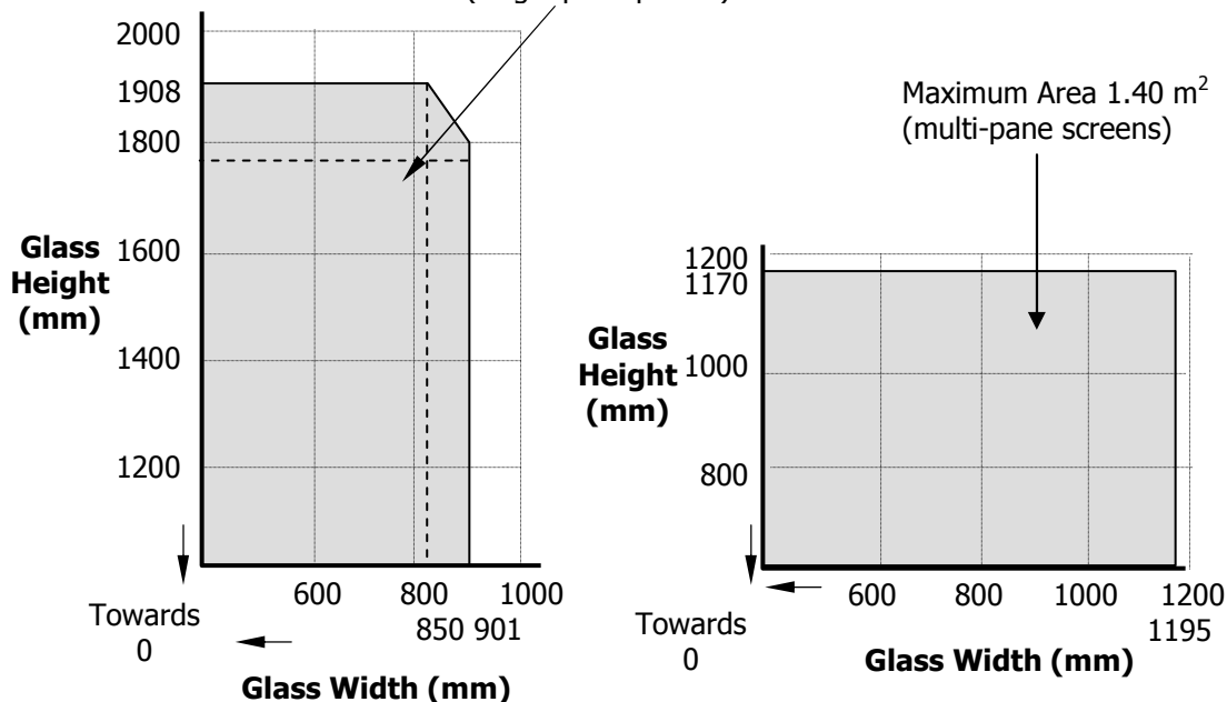
Figure 6. Maximum Permitted Glass Dimensions
