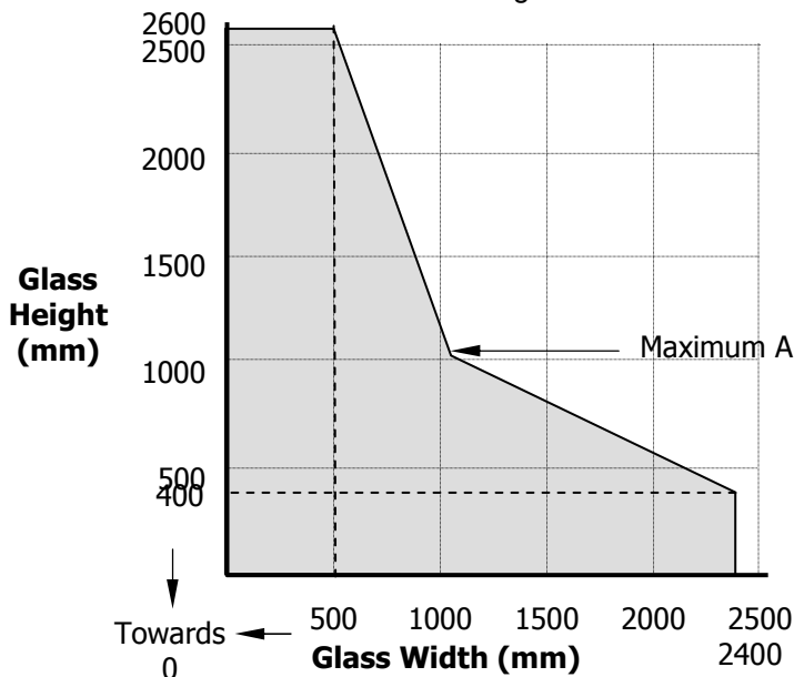
Figure 4. Maximum Permitted Glass Dimensions
