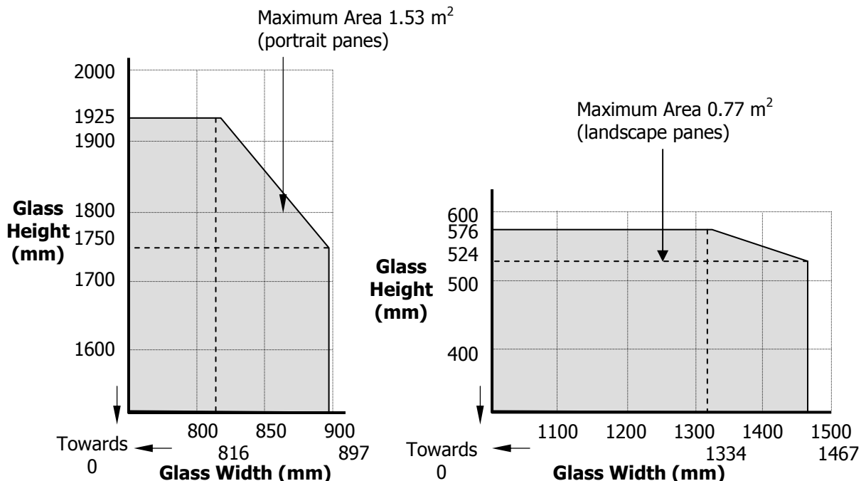
Figure 7. Maximum Permitted Glass Dimensions
