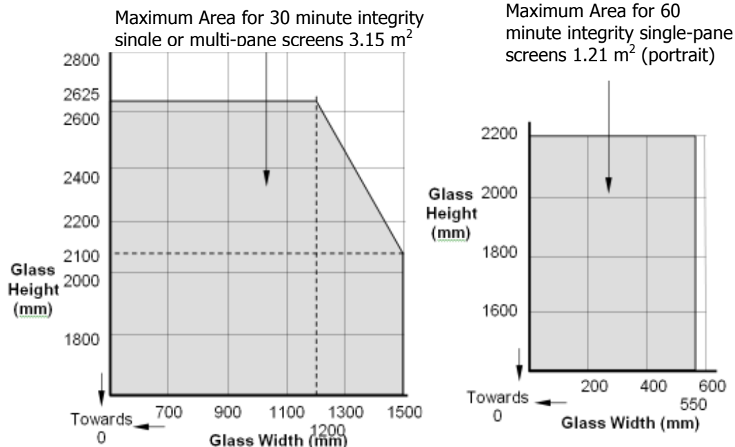
Figure 8. Maximum Permitted Glass Dimensions
